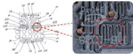
Patented PCB circuit provides excellent work in easing internal magent coupling to 500MHz
